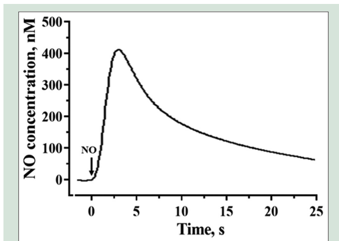
Figure 1: Amperometric curve showing response of nitric oxide sensor to 400 nM concentration of standard nitric oxide solution (Hank's balanced salt solution buffer)
